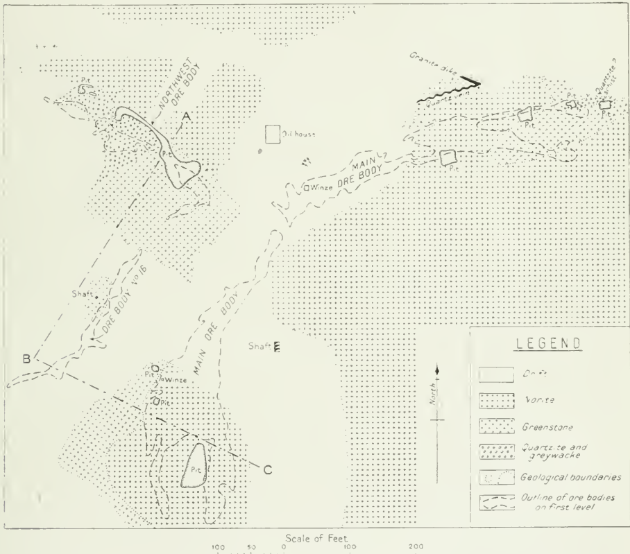
Fig. 31—Geological map of Garson mine, showing outline of ore bodies on first level, and location of cross-section A B C, Sudbury area, Ontario.
